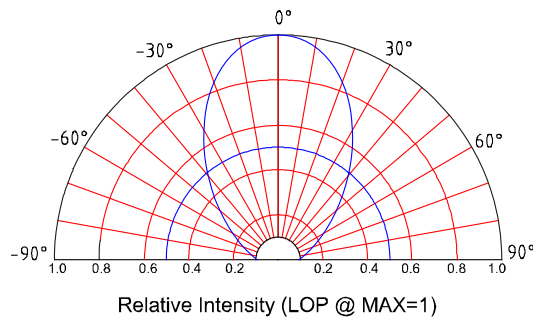
Beam Patter
